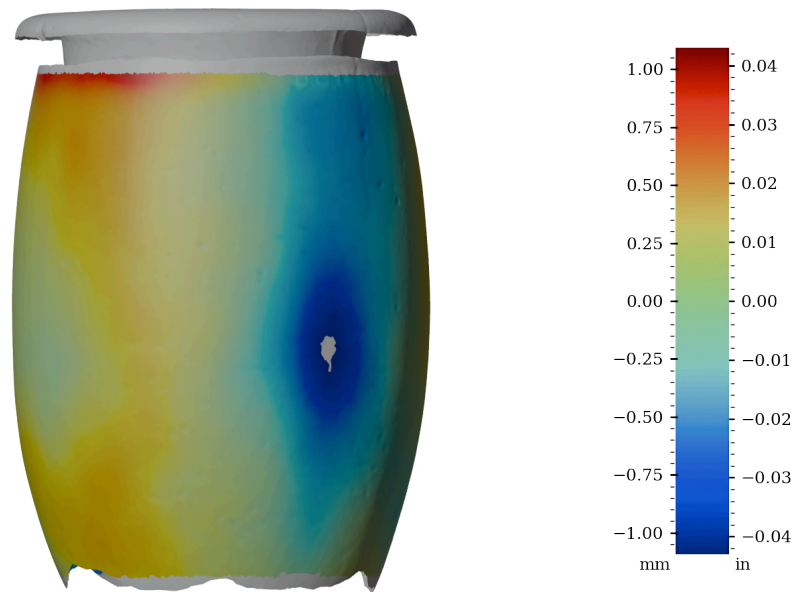
Figure 48: Surface variability heatmap of MV031, rotated 270°
