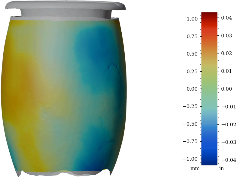
Figure 46: Surface variability heatmap of MV031, rotated 90°
