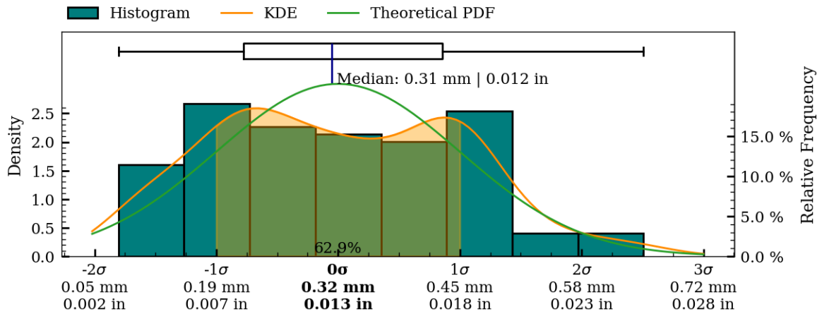
Figure 44: Coaxiality residual plots of interior_separate surface, MV031.
