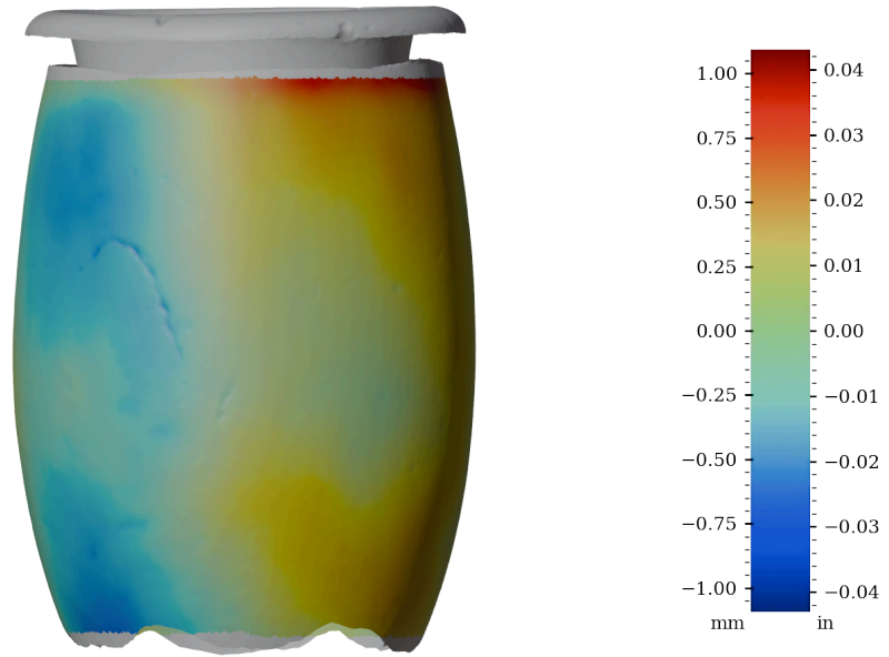
Figure 47: Surface variability heatmap of MV031, rotated 180°
