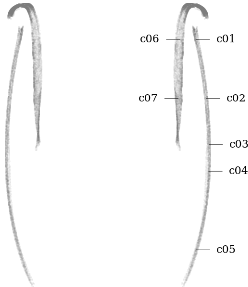
Figure 31: Circularity measurement sample locations, full mesh aligned to exterior surface
