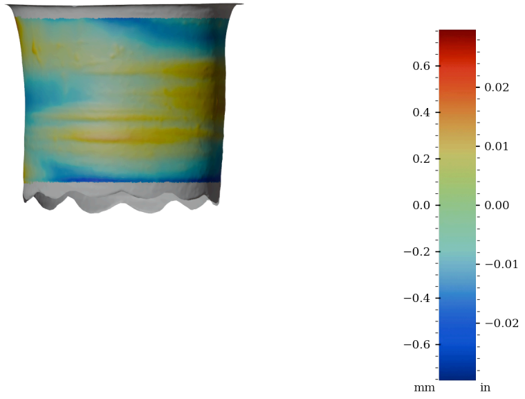
Figure 55: Surface variability heatmap of MV031, rotated 180°
