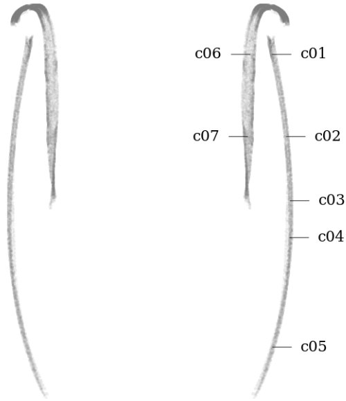
Figure 62: Circularity measurement sample locations, full mesh aligned to exterior surface
