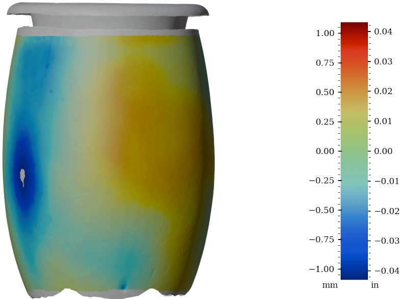
Figure 45: Surface variability heatmap of MV031, front view
