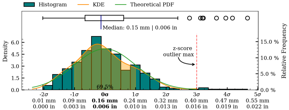
Figure 42: Coaxiality residual plots of exterior surface, MV031.
