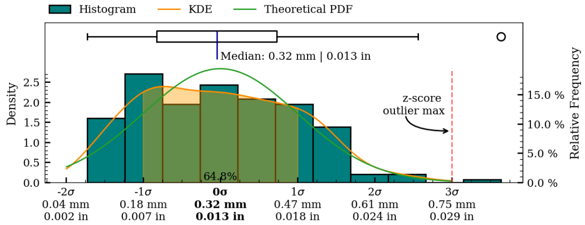
Figure 43: Coaxiality residual plots of interior surface, MV031.
