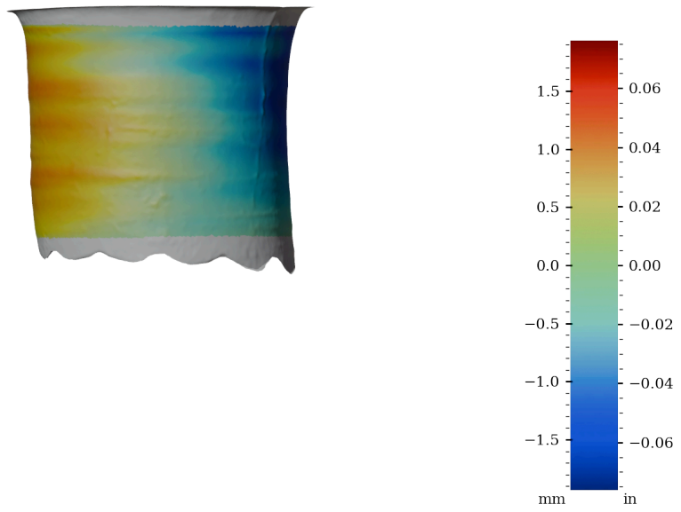
Figure 52: Surface variability heatmap of MV031, rotated 270°
