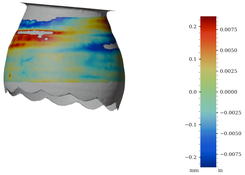
Figure 57: Surface variability heatmap of MV028, front view
