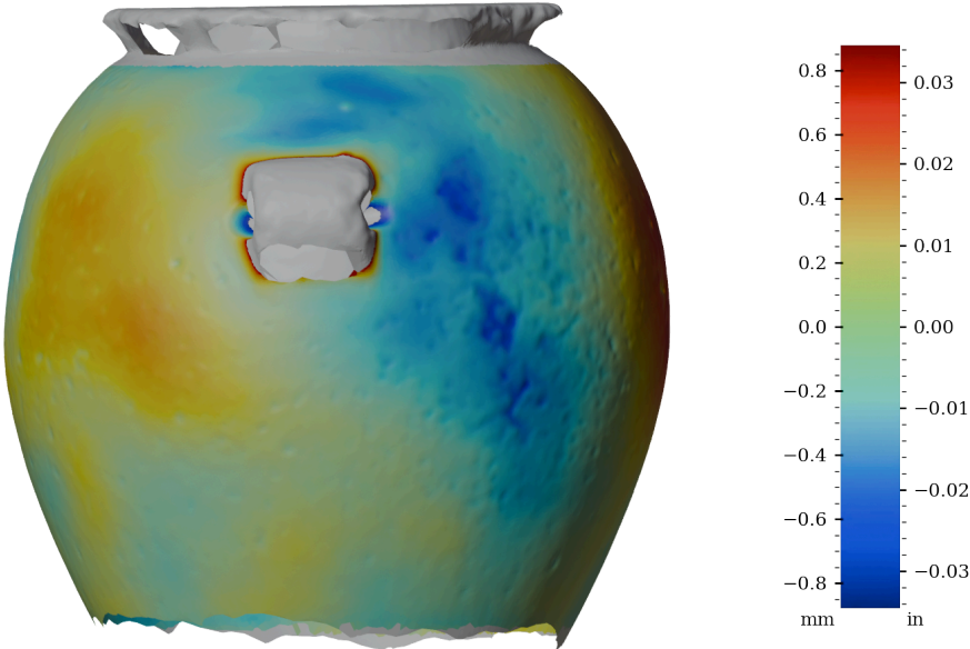
Figure 50: Surface variability heatmap of MV028, rotated 90°
