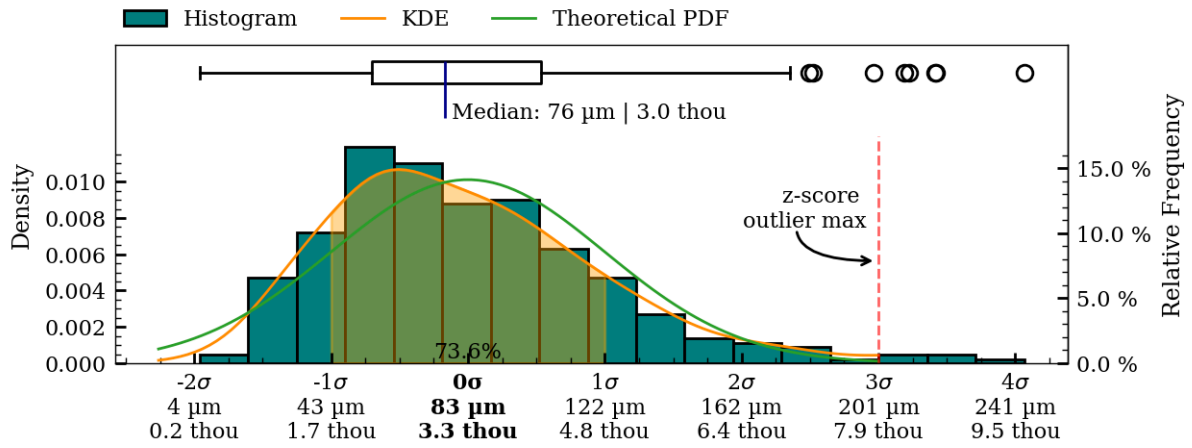
Figure 46: Coaxiality residual plots of exterior surface, MV028.
