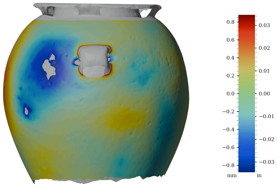
Figure 52: Surface variability heatmap of MV028, rotated 270°
