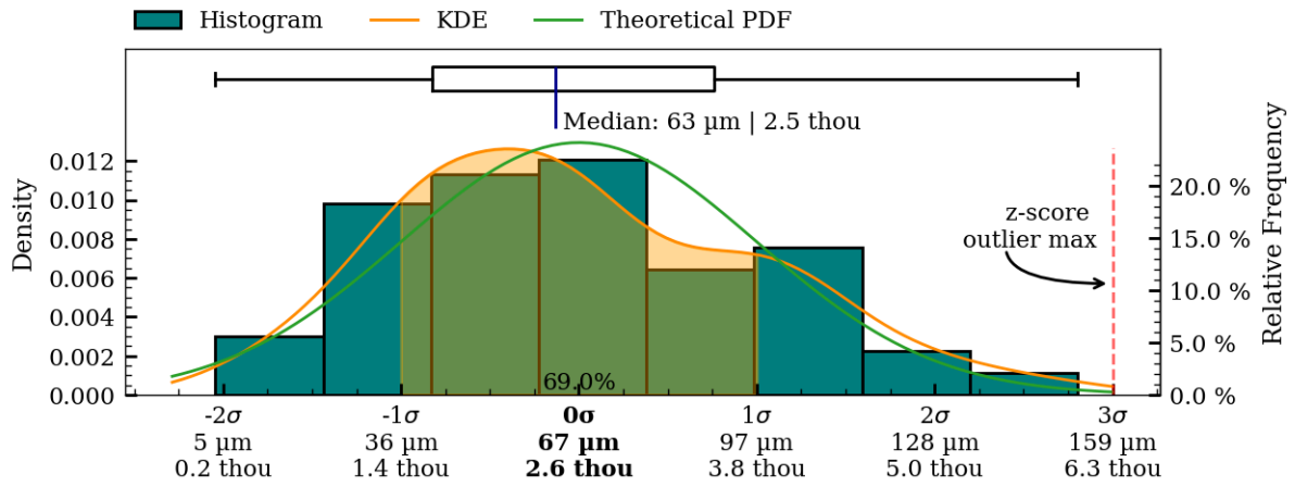
Figure 47: Coaxiality residual plots of interior surface, MV028.
