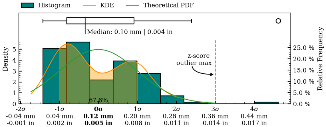
Figure 48: Coaxiality residual plots of interior_separate surface, MV028.
