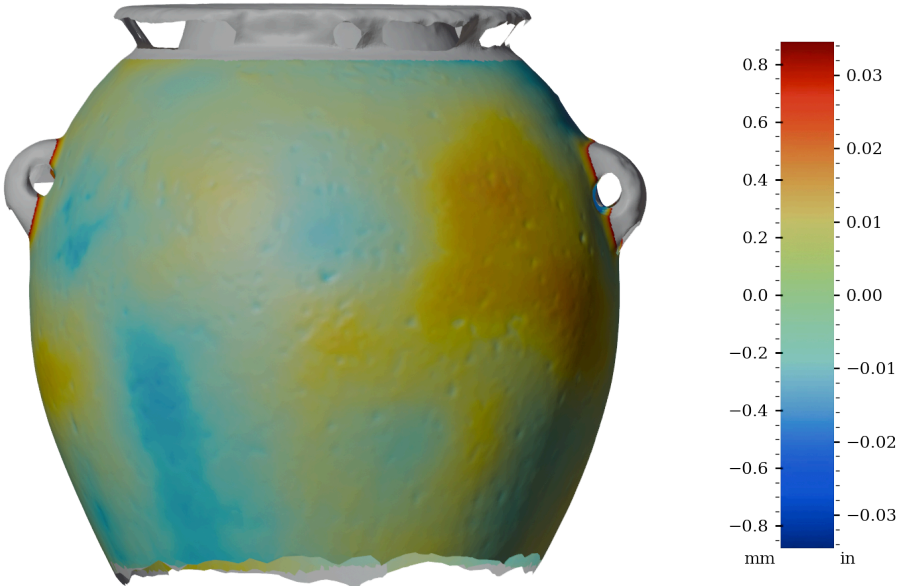
Figure 49: Surface variability heatmap of MV028, front view
