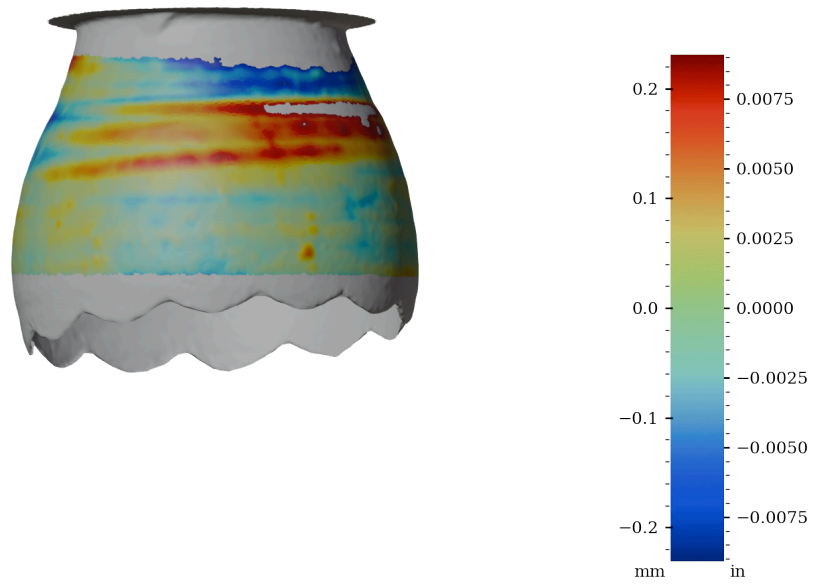
Figure 60: Surface variability heatmap of MV028, rotated 270°
