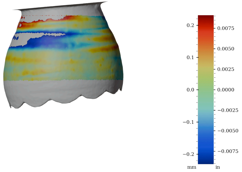
Figure 59: Surface variability heatmap of MV028, rotated 180°
