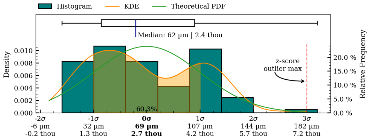
Figure 51: Coaxiality residual plots of interior surface, MV027.
