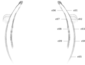
Figure 35: Circularity measurement sample locations, full mesh aligned to exterior surface
