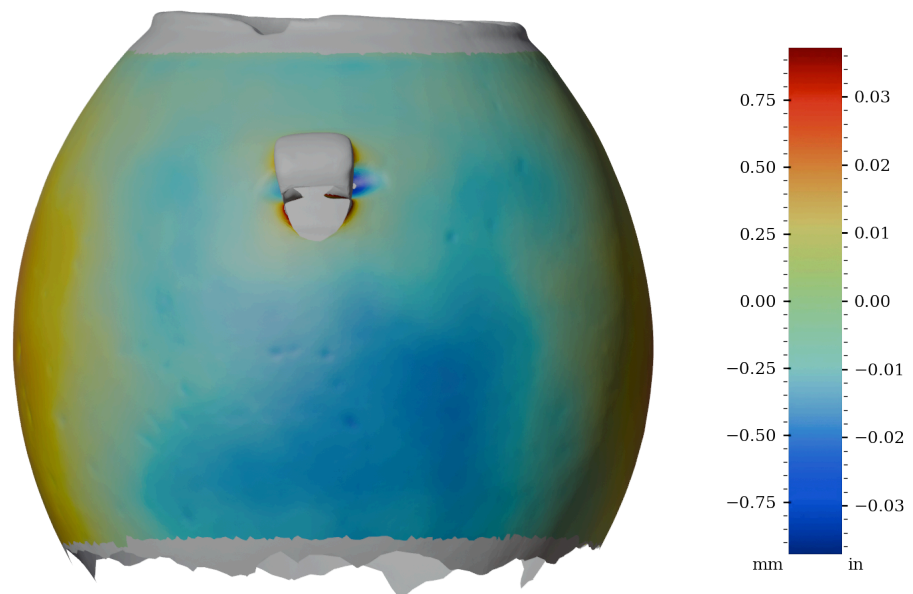
Figure 56: Surface variability heatmap of MV027, rotated 270°
