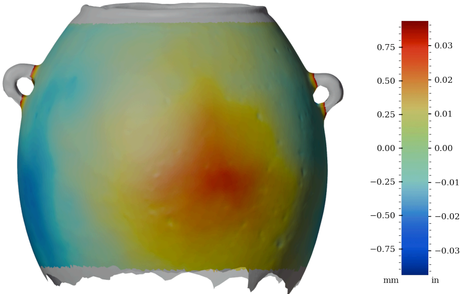
Figure 53: Surface variability heatmap of MV027, front view
