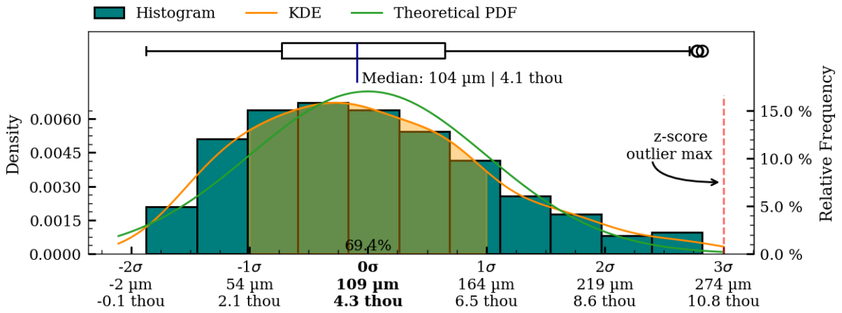
Figure 50: Coaxiality residual plots of exterior surface, MV027.
