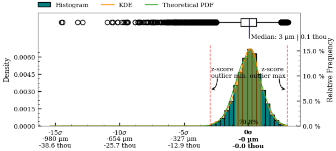
Figure 67: Interior separately aligned surface variability boxplot, kds and histogram.
