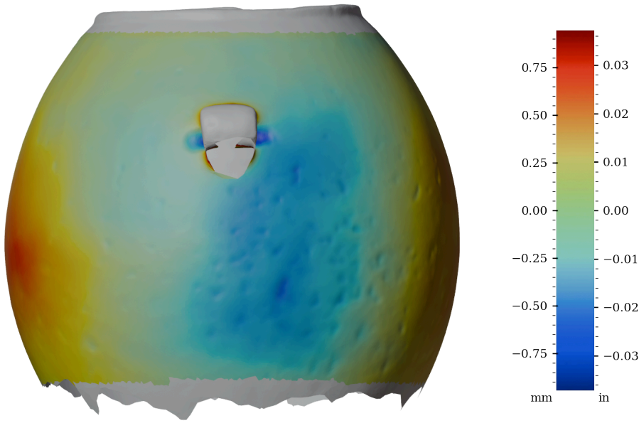
Figure 54: Surface variability heatmap of MV027, rotated 90°
