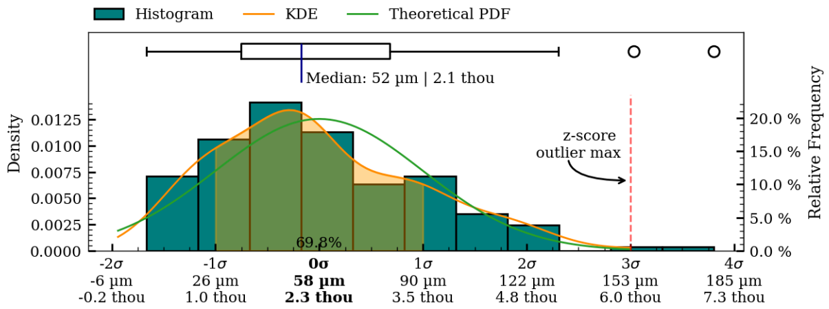
Figure 52: Coaxiality residual plots of interior_separate surface, MV027.
