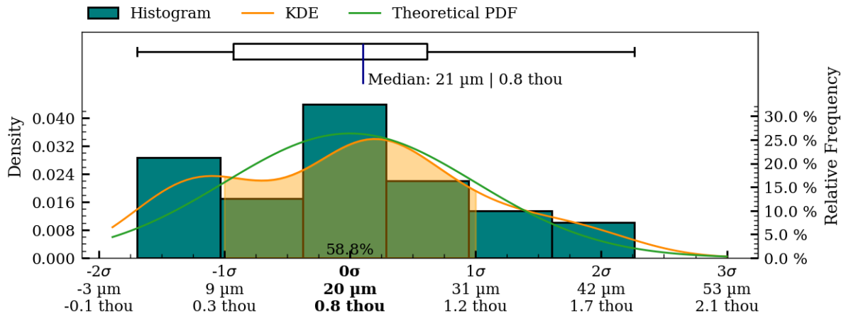
Figure 44: Coaxiality residual plots of interior_separate surface, MV026.
