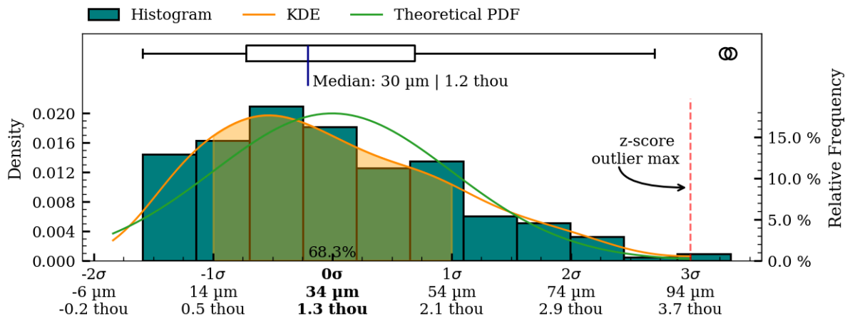
Figure 42: Coaxiality residual plots of exterior surface, MV026.
