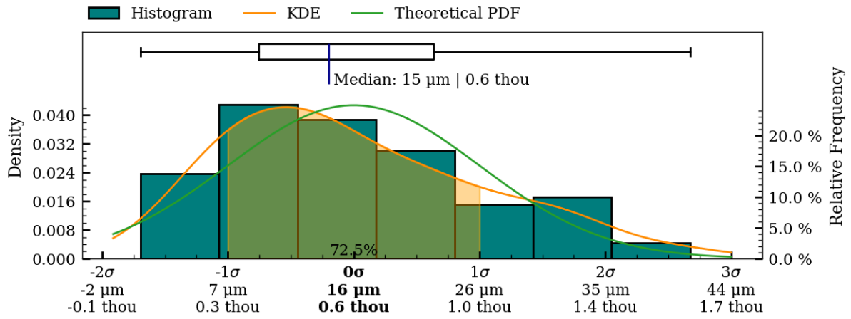
Figure 43: Coaxiality residual plots of interior surface, MV026.
