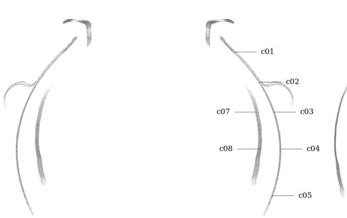
Figure 76: Circularity measurement sample locations, full mesh aligned to exterior surface
