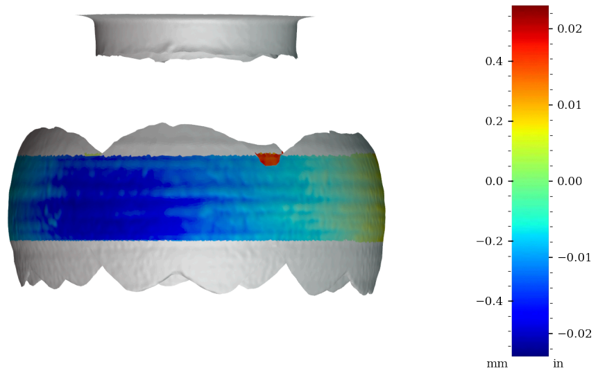
Figure 50: Surface variability heatmap of MV026, rotated 90°
