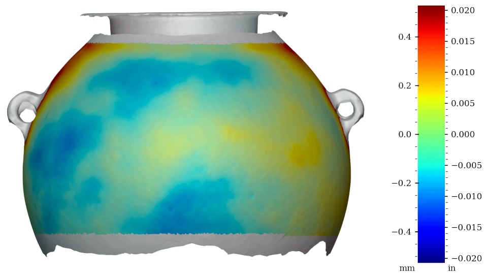
Figure 45: Surface variability heatmap of MV026, front view
