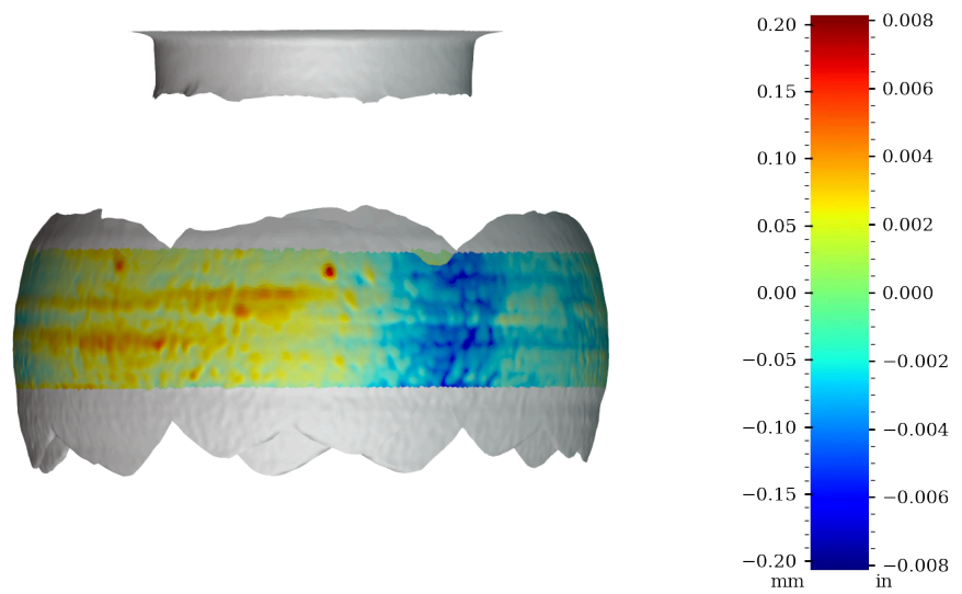
Figure 56: Surface variability heatmap of MV026, rotated 270°
