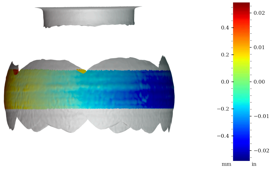
Figure 49: Surface variability heatmap of MV026, front view
