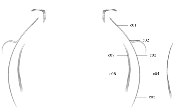
Figure 60: Circularity measurement sample locations, full mesh aligned to exterior surface
