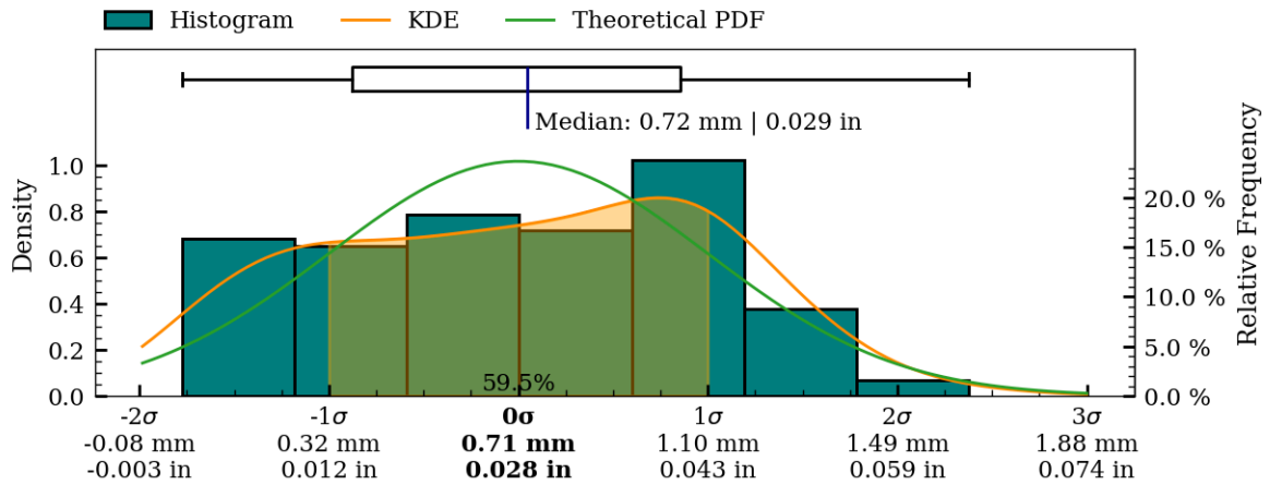
Figure 47: Coaxiality residual plots of interior surface, MV025.
