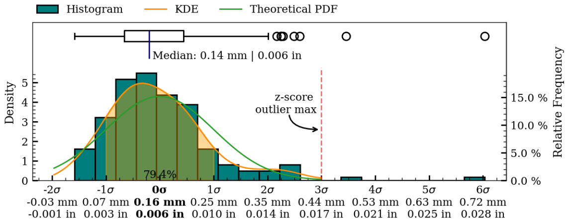
Figure 46: Coaxiality residual plots of exterior surface, MV025.
