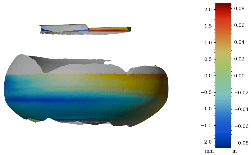
Figure 53: Surface variability heatmap of MV025, front view
