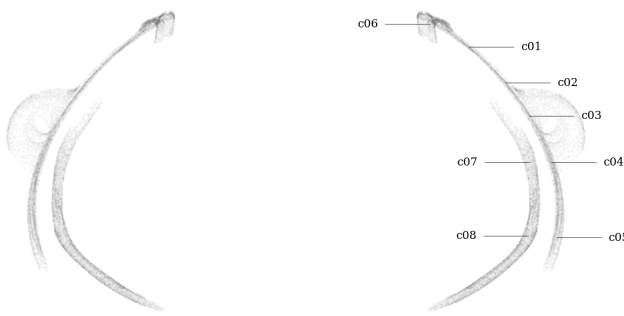
Figure 82: Circularity measurement sample locations, full mesh aligned to exterior surface
