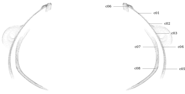
Figure 33: Circularity measurement sample locations, full mesh aligned to exterior surface
