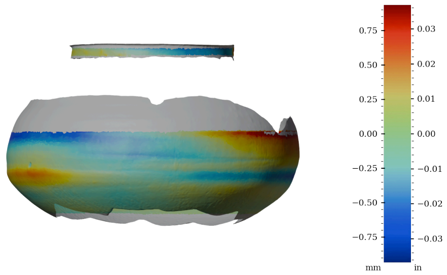
Figure 60: Surface variability heatmap of MV025, rotated 270°
