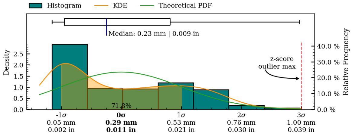
Figure 48: Coaxiality residual plots of interior_separate surface, MV025.
