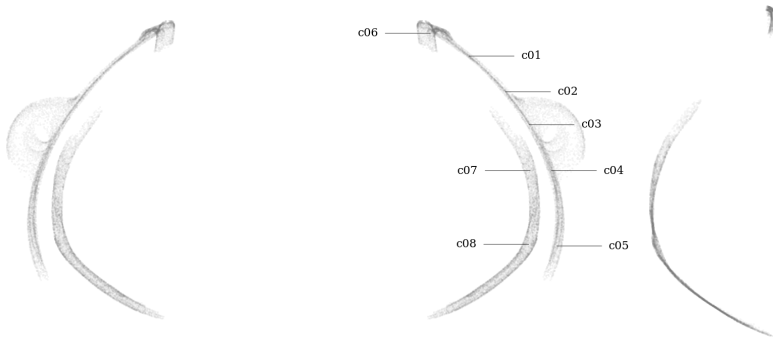
Figure 80: Circularity measurement sample locations, full mesh aligned to exterior surface
