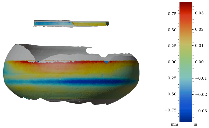
Figure 57: Surface variability heatmap of MV025, front view
