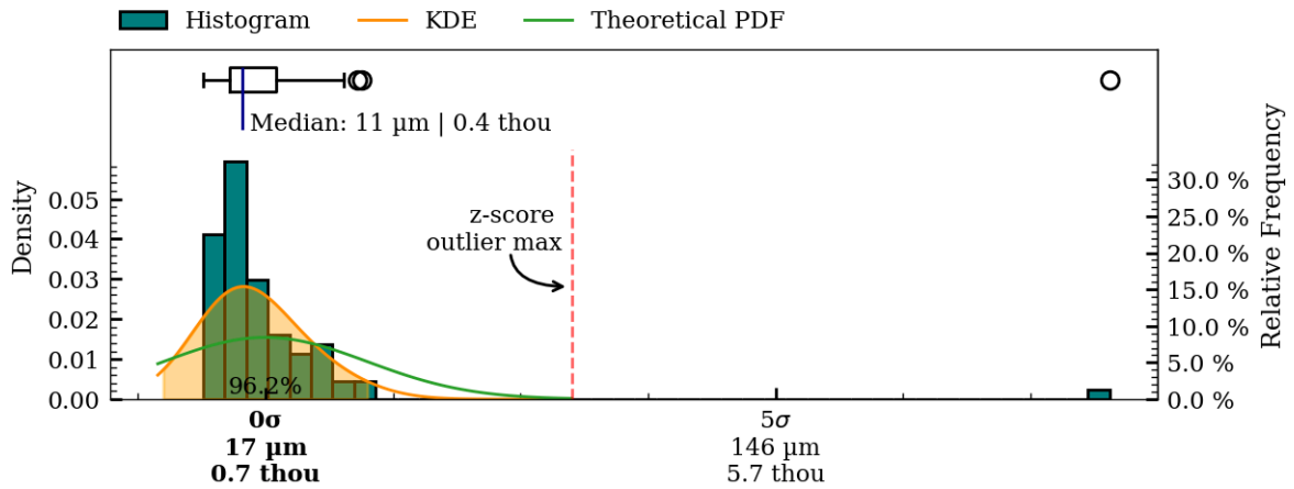
Figure 39: Coaxiality residual plots of interior surface, MV005.
