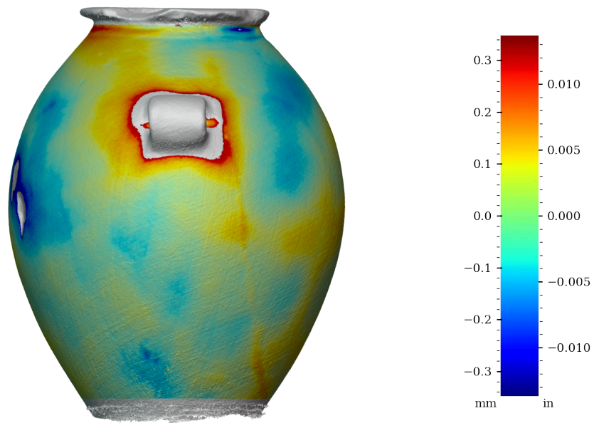
Figure 44: Surface variability heatmap of MV005, rotated 270°
