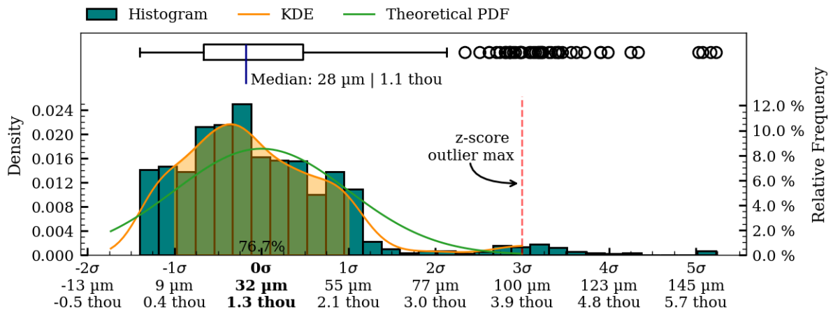
Figure 38: Coaxiality residual plots of exterior surface, MV005.
