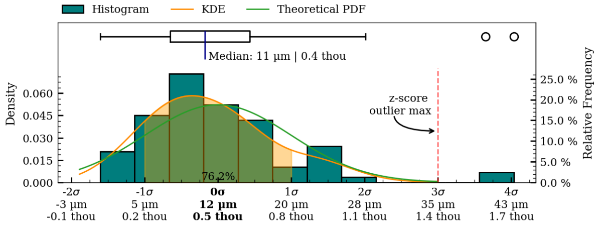
Figure 40: Coaxiality residual plots of interior_separate surface, MV005.
