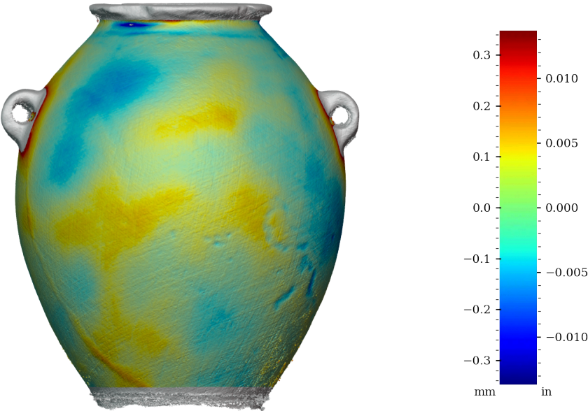
Figure 41: Surface variability heatmap of MV005, front view
