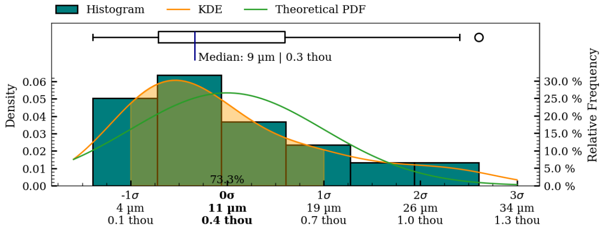
Figure 40: Coaxiality residual plots of interior_separate surface, MV004.
