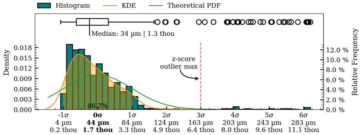
Figure 38: Coaxiality residual plots of exterior surface, MV004.
