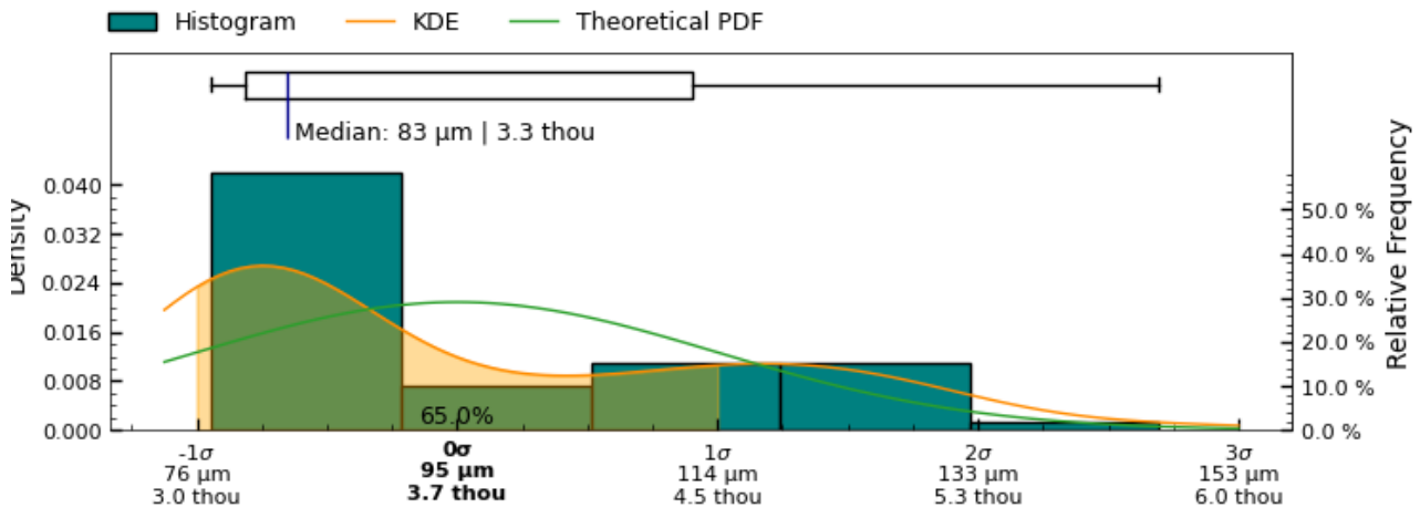
Figure 27: Root Mean Squared Deviation measurement distribution across measured slices of interior separately aligned surface
