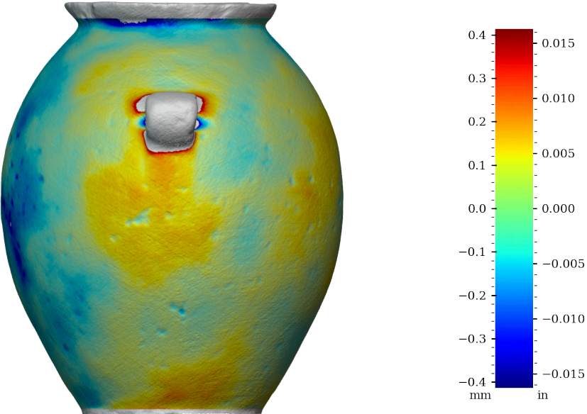
Figure 42: Surface variability heatmap of MV004, rotated 90°
