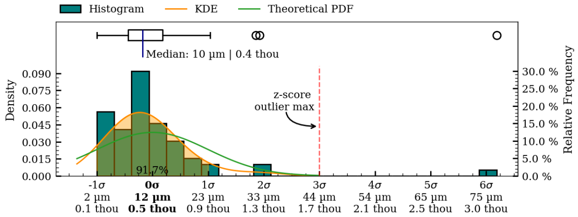
Figure 39: Coaxiality residual plots of interior surface, MV004.
