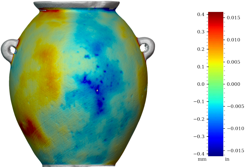
Figure 41: Surface variability heatmap of MV004, front view
