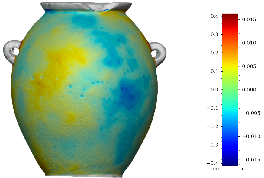
Figure 43: Surface variability heatmap of MV004, rotated 180°
