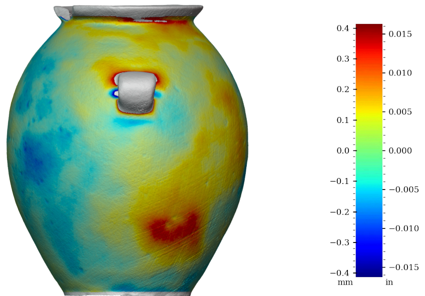
Figure 44: Surface variability heatmap of MV004, rotated 270°
