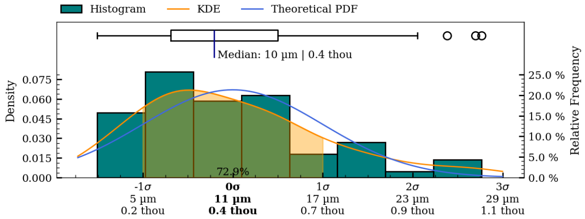
Figure 43: Coaxiality residual plots of interior surface, IV006.
