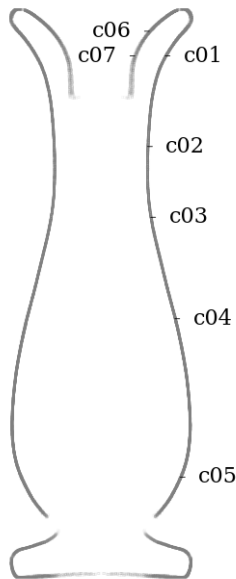
Figure 31: Circularity measurement sample locations, full mesh aligned to exterior surface
