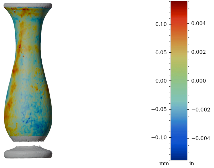
Figure 48: Surface variability heatmap of IV006, rotated 270°
