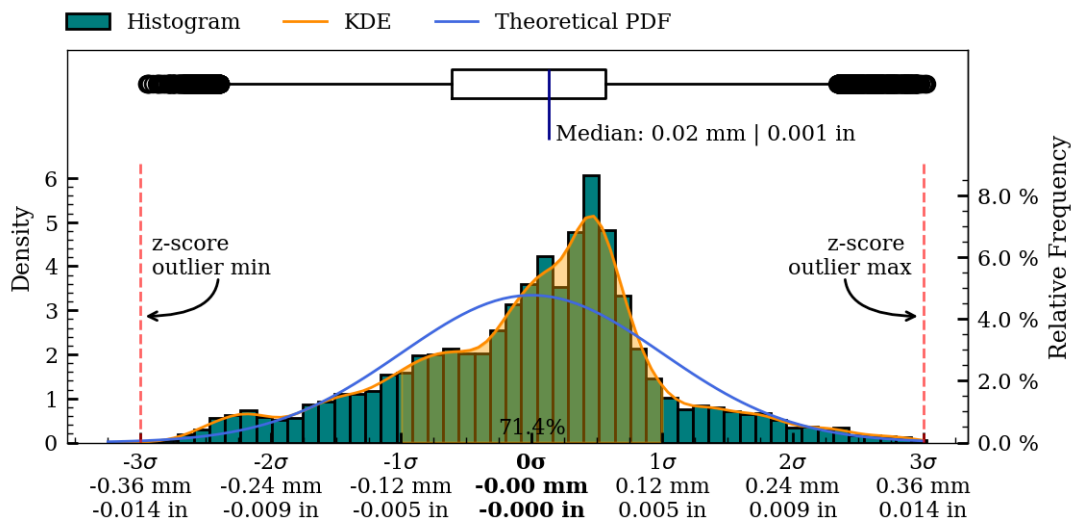
Figure 58: Interior surface variability boxplot, kds and histogram.
