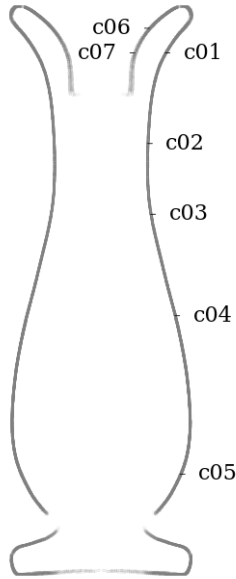
Figure 62: Circularity measurement sample locations, full mesh aligned to exterior surface
