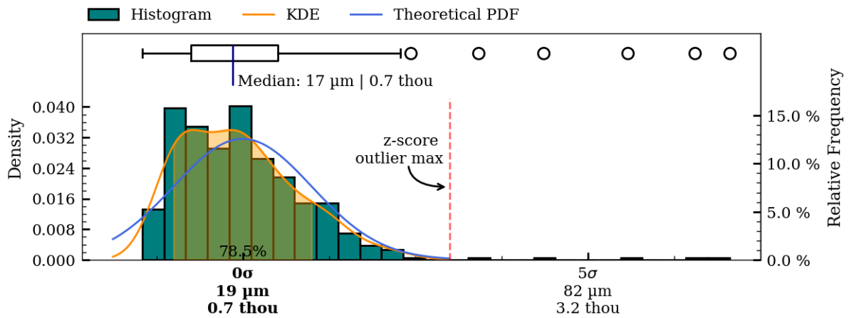
Figure 42: Coaxiality residual plots of exterior surface, IV006.
