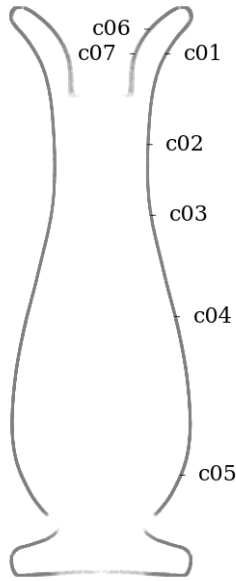
Figure 78: Circularity measurement sample locations, full mesh aligned to exterior surface
