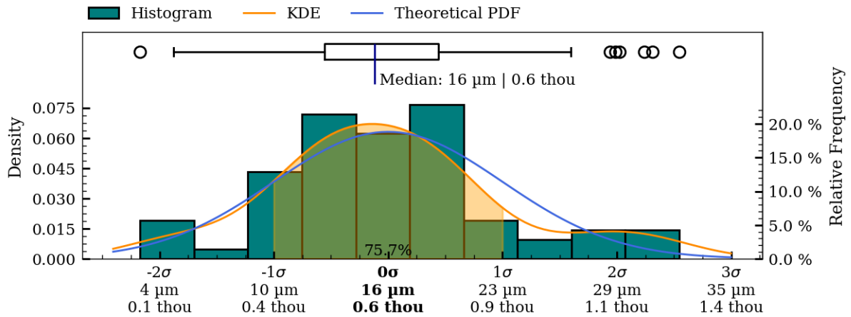
Figure 44: Coaxiality residual plots of interior_separate surface, IV006.
