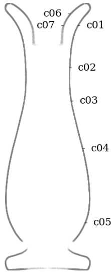
Figure 76: Circularity measurement sample locations, full mesh aligned to exterior surface
