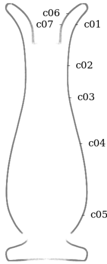
Figure 4: Circularity measurement sample locations, full mesh aligned with exterior surface
