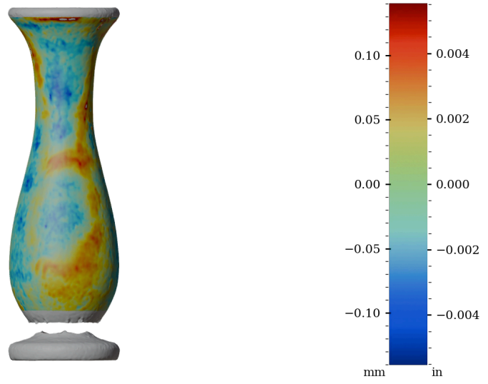
Figure 47: Surface variability heatmap of IV006, rotated 180°
