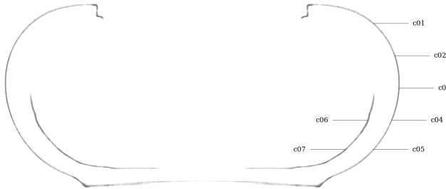
Figure 60: Circularity measurement sample locations, full mesh aligned to exterior surface
