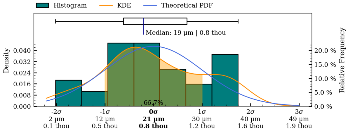
Figure 44: Coaxiality residual plots of interior_separate surface, IV005.
