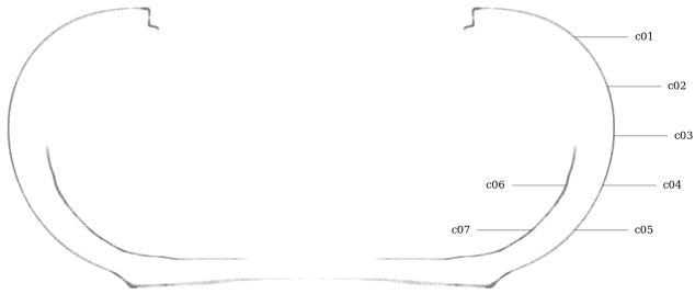
Figure 31: Circularity measurement sample locations, full mesh aligned to exterior surface
