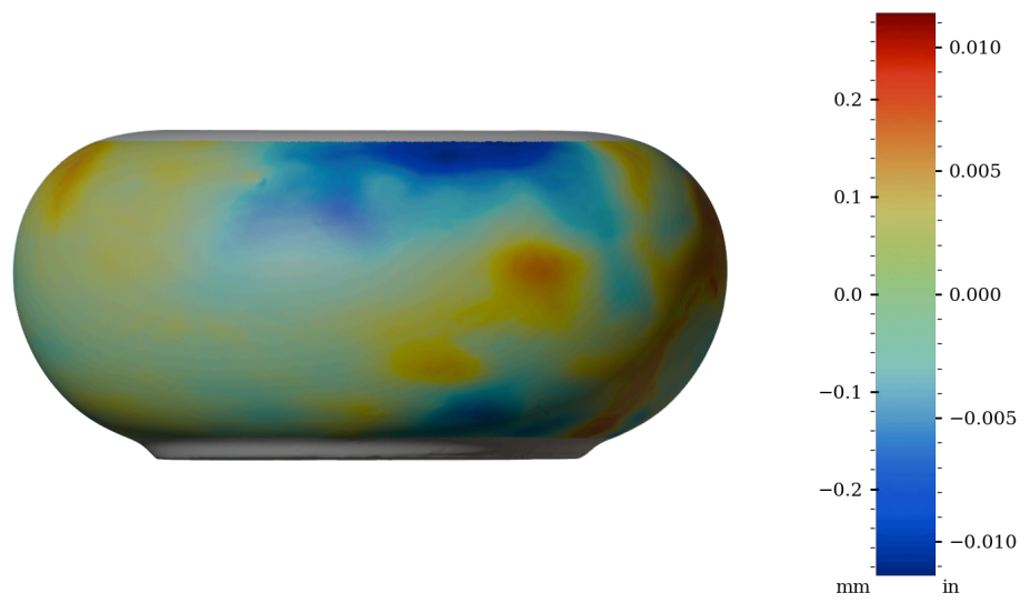
Figure 48: Surface variability heatmap of IV005, rotated 270°
