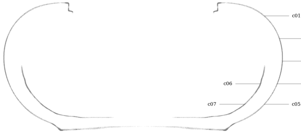
Figure 76: Circularity measurement sample locations, full mesh aligned to exterior surface
