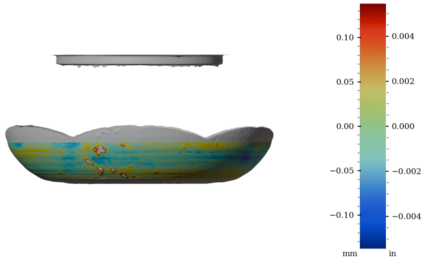
Figure 53: Surface variability heatmap of IV005, front view
