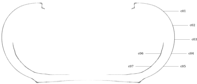
Figure 78: Circularity measurement sample locations, full mesh aligned to exterior surface
