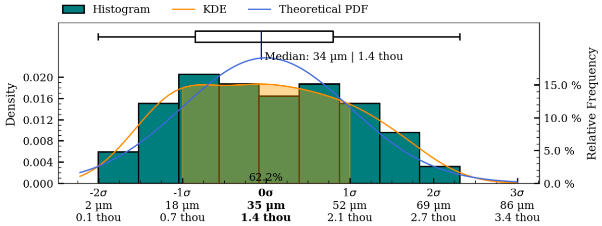
Figure 42: Coaxiality residual plots of exterior surface, IV005.
