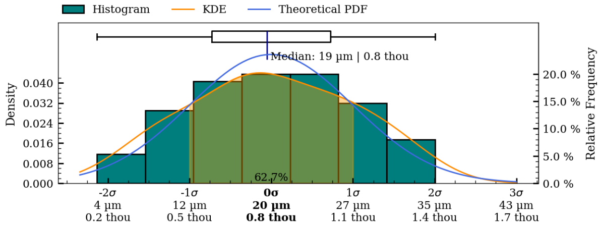
Figure 43: Coaxiality residual plots of interior surface, IV005.
