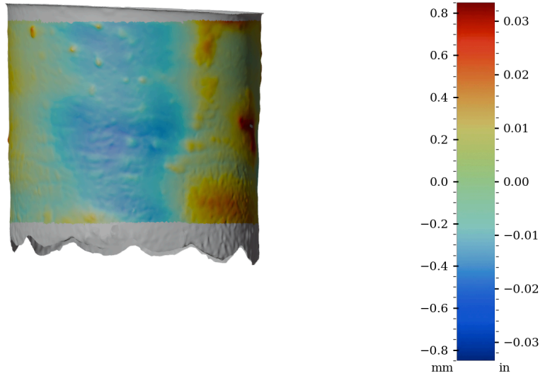
Figure 56: Surface variability heatmap of HV008, rotated 270°
