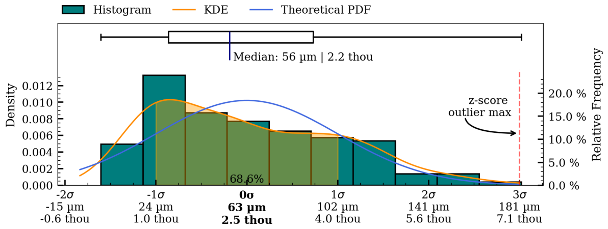
Figure 44: Coaxiality residual plots of interior_separate surface, HV008.
