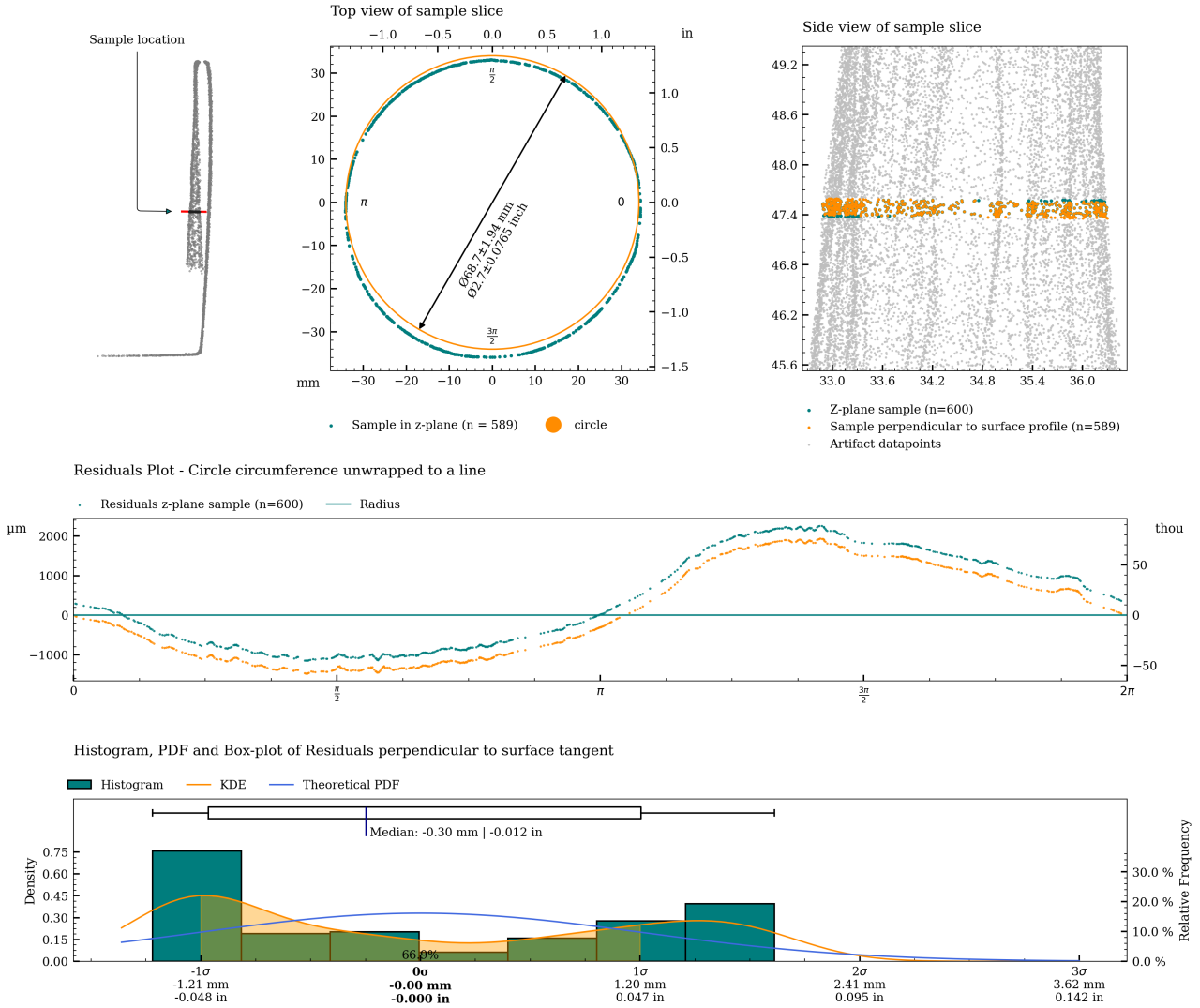
Figure 14: Charts with statistics for the measurement of c09.
