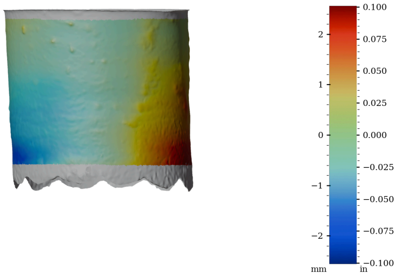
Figure 52: Surface variability heatmap of HV008, rotated 270°
