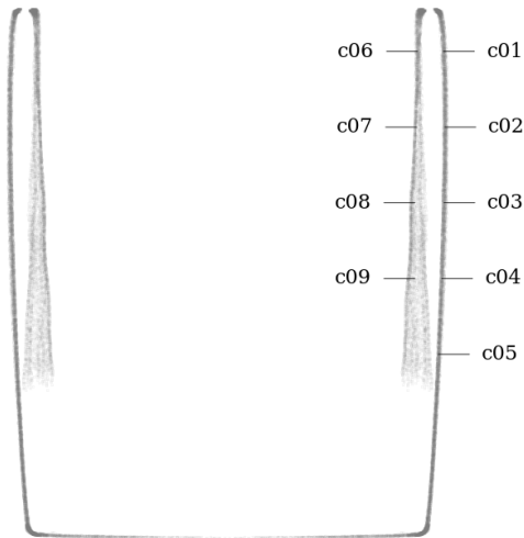
Figure 31: Circularity measurement sample locations, full mesh aligned to exterior surface
