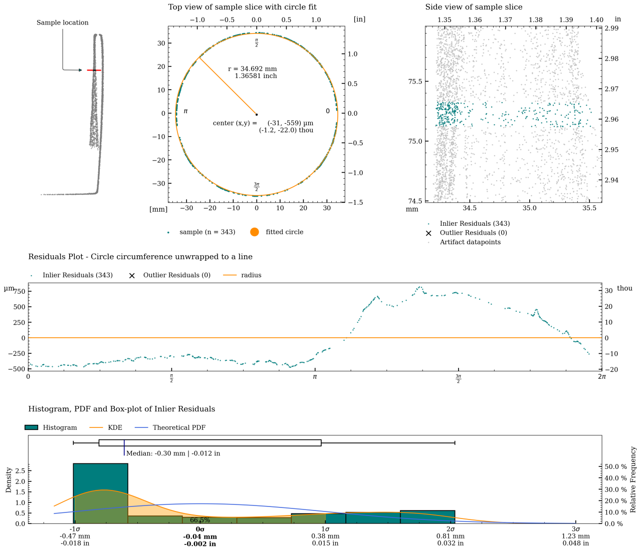
Figure 39: Detailed plot of concentricity measurement for c07.
