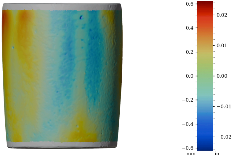
Figure 48: Surface variability heatmap of HV008, rotated 270°
