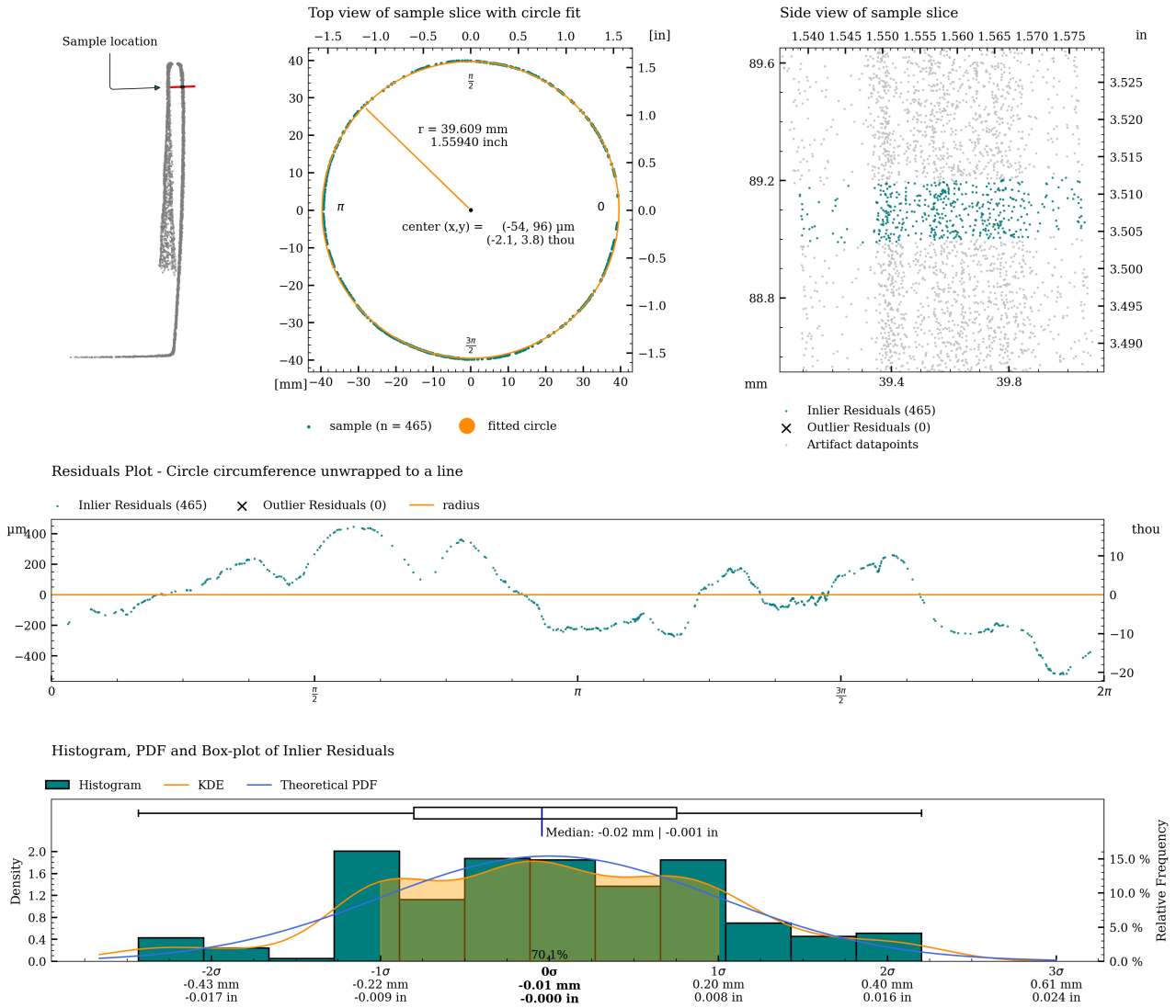
Figure 33: Detailed plot of concentricity measurement for c01.
