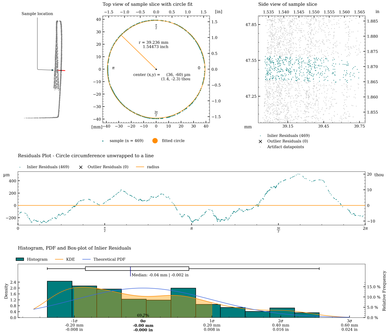
Figure 36: Detailed plot of concentricity measurement for c04.
