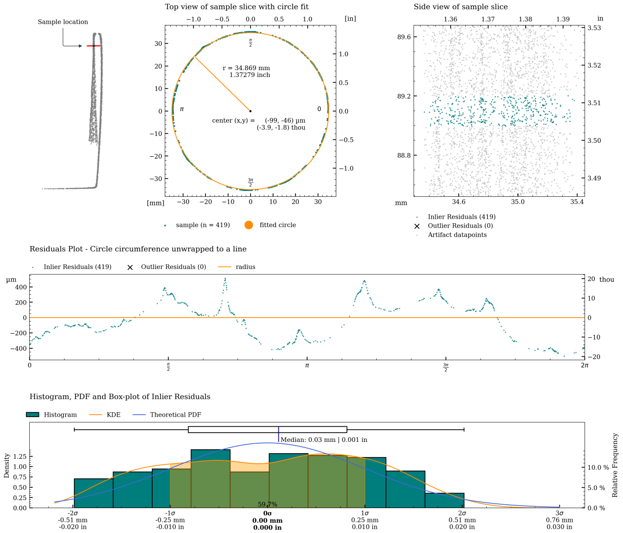
Figure 38: Detailed plot of concentricity measurement for c06.
