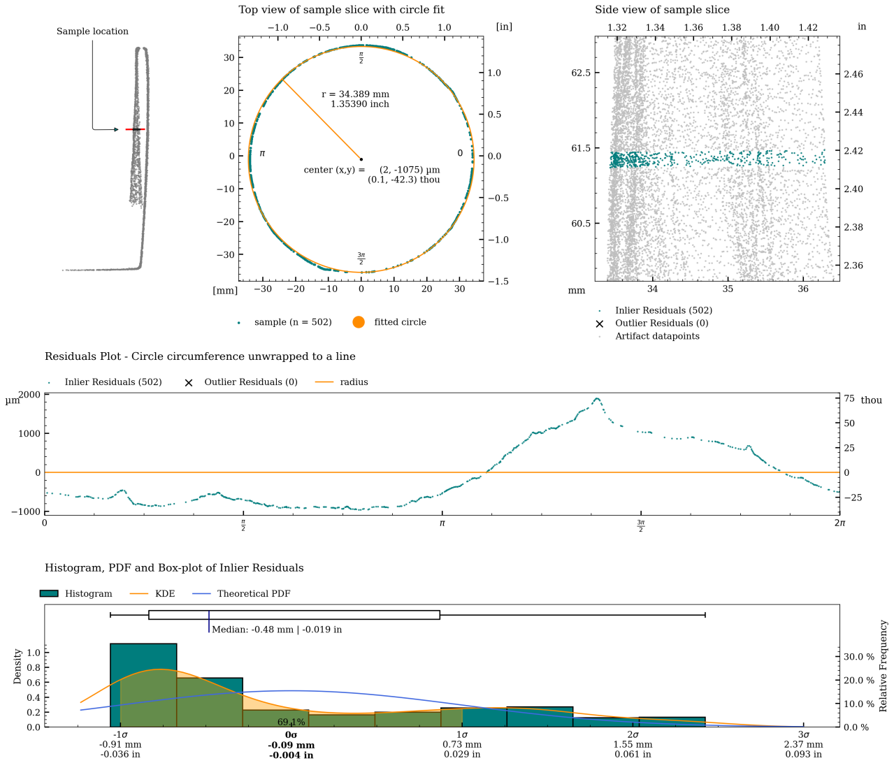
Figure 40: Detailed plot of concentricity measurement for c08.
