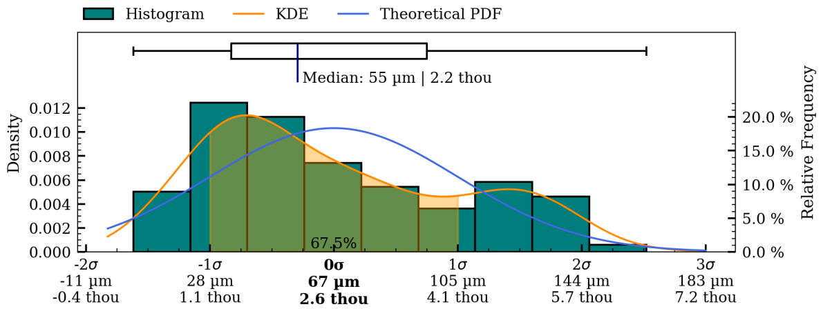
Figure 43: Coaxiality residual plots of interior surface, HV008.
