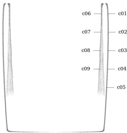
Figure 78: Circularity measurement sample locations, full mesh aligned to exterior surface
