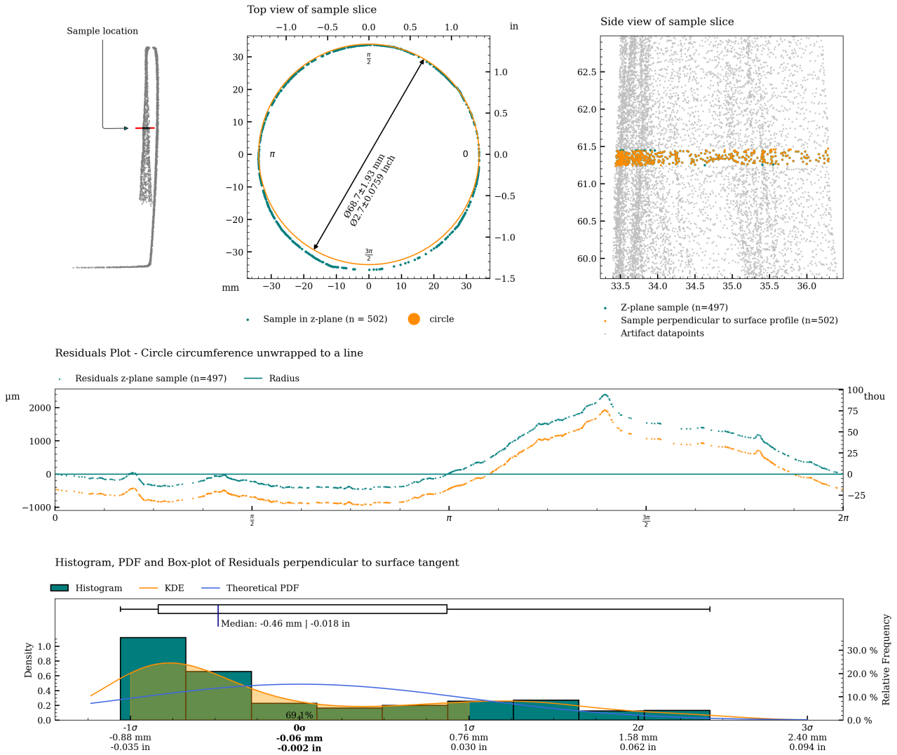
Figure 13: Charts with statistics for the measurement of c08.
