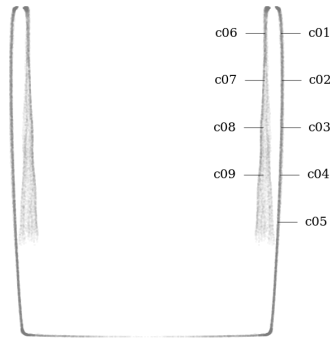
Figure 76: Circularity measurement sample locations, full mesh aligned to exterior surface
