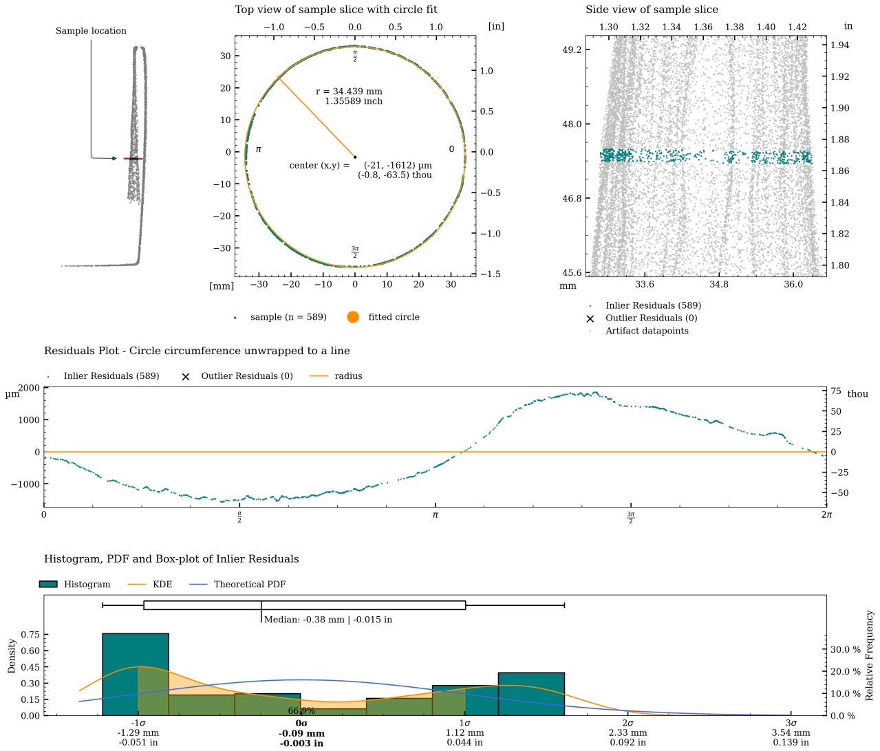
Figure 41: Detailed plot of concentricity measurement for c09.
