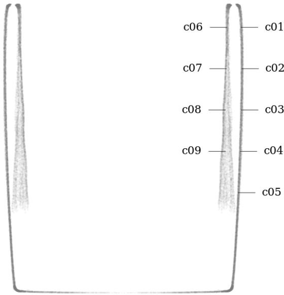
Figure 60: Circularity measurement sample locations, full mesh aligned to exterior surface
