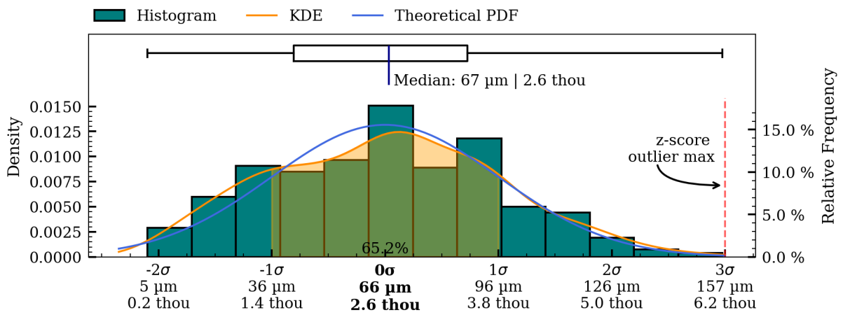
Figure 42: Coaxiality residual plots of exterior surface, HV008.
